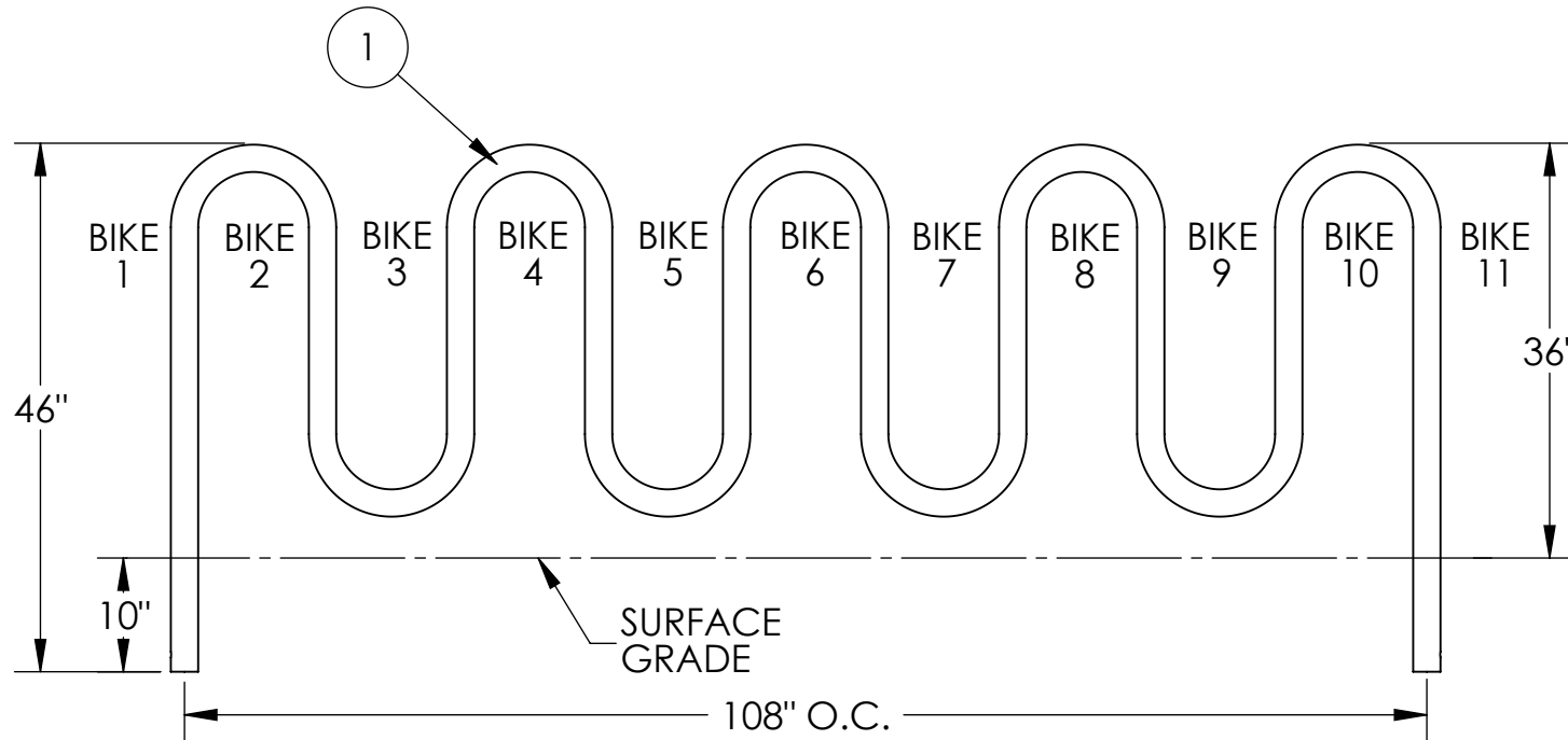
FRONT VIEW
